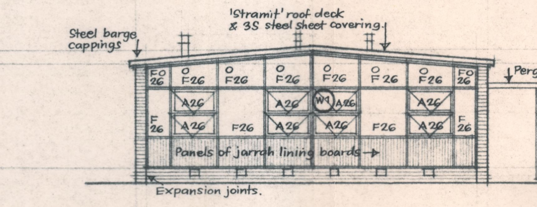
NORTH ELEVATION
