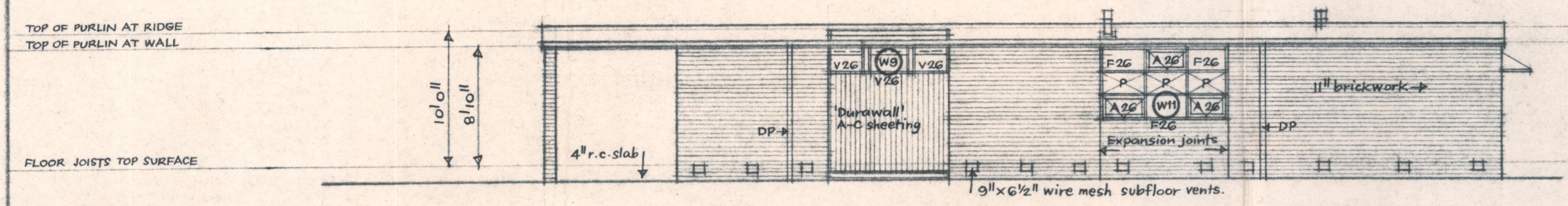
EAST ELEVATION
