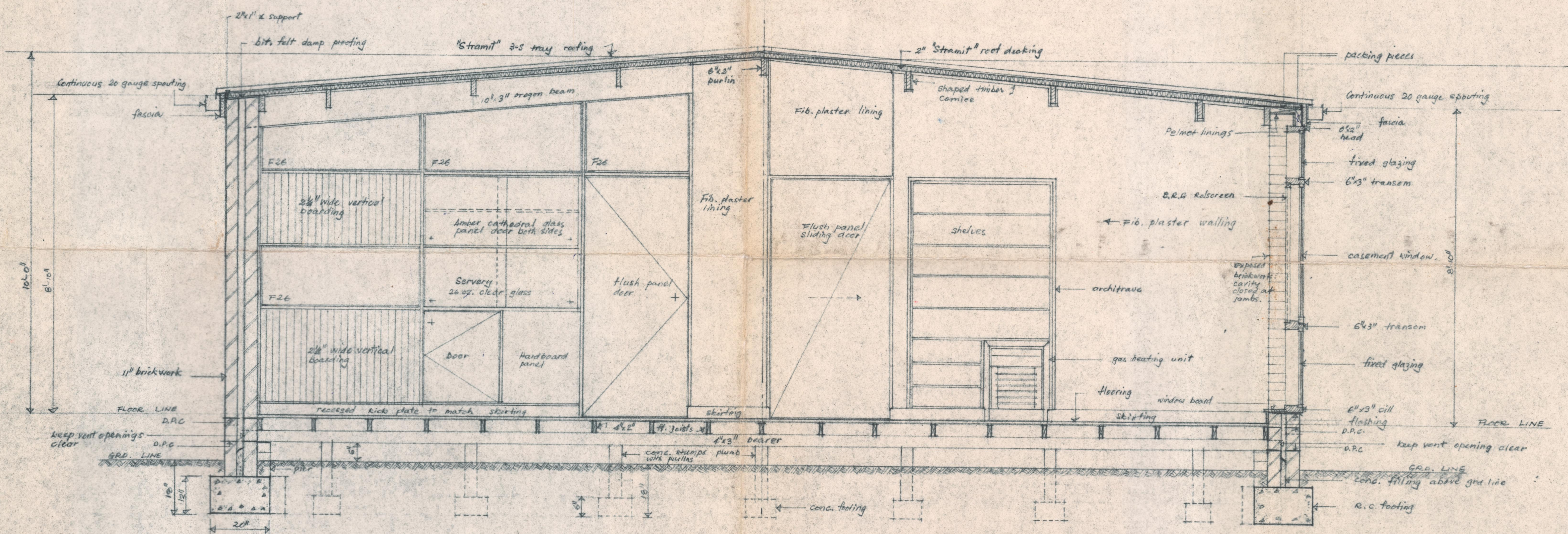
DETAILED SECTION THROUGH LOUNGE & DINING ROOM LOOKING SOUTH
