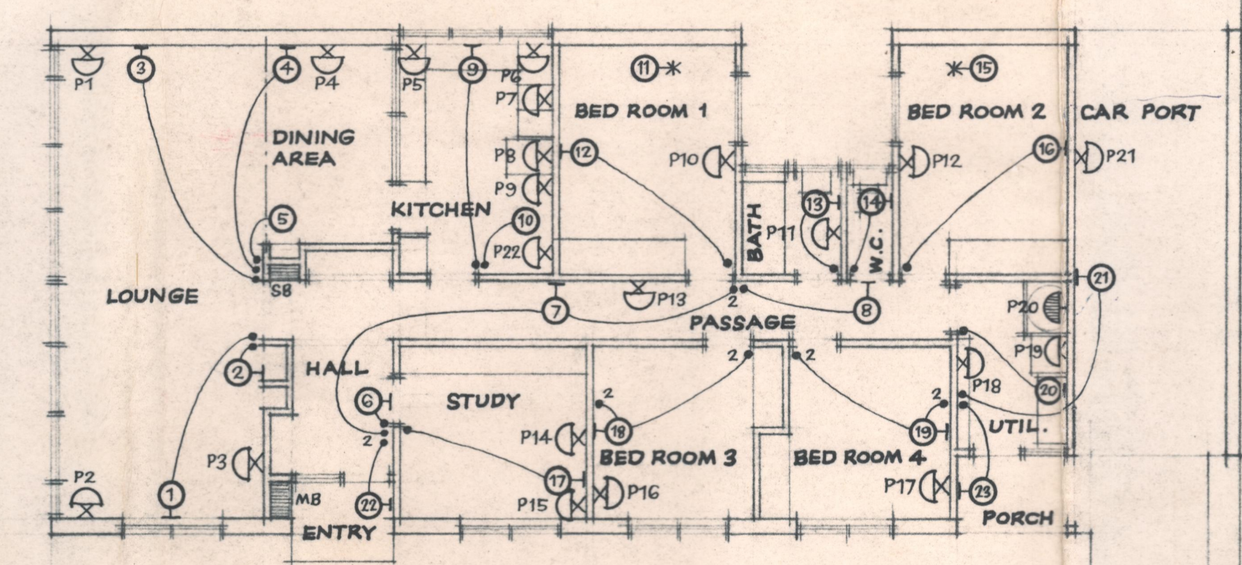
ELECTRICAL PLAN
