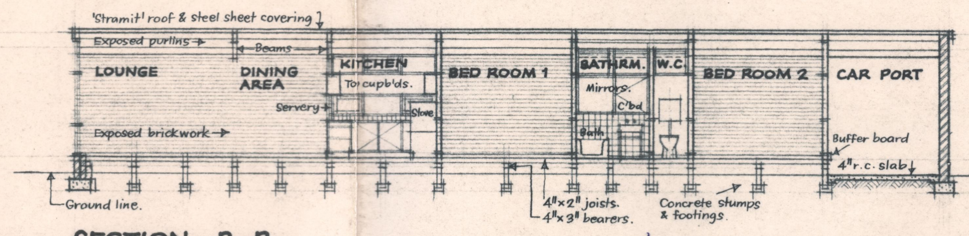
SECTION B-B
