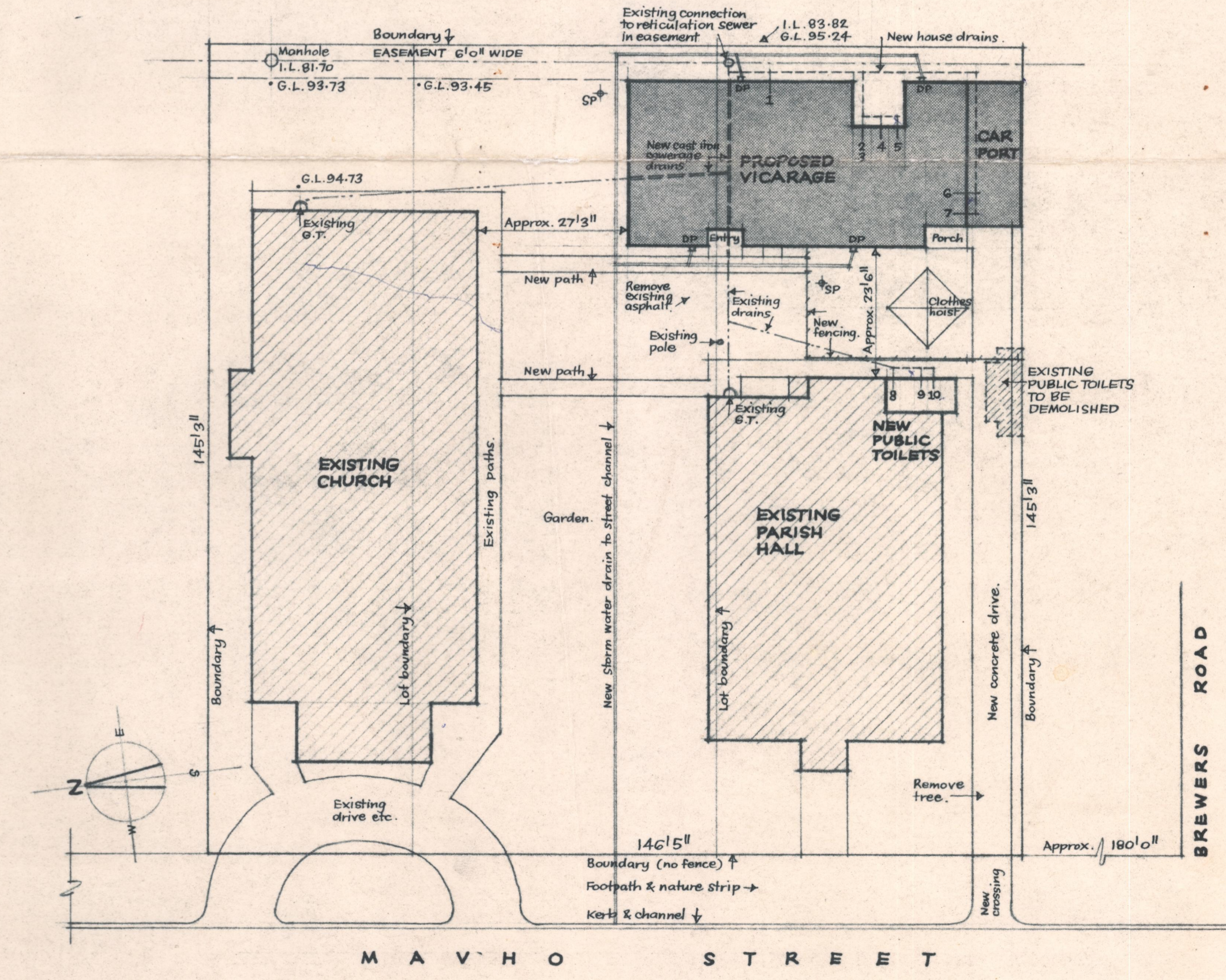
SITE PLAN
