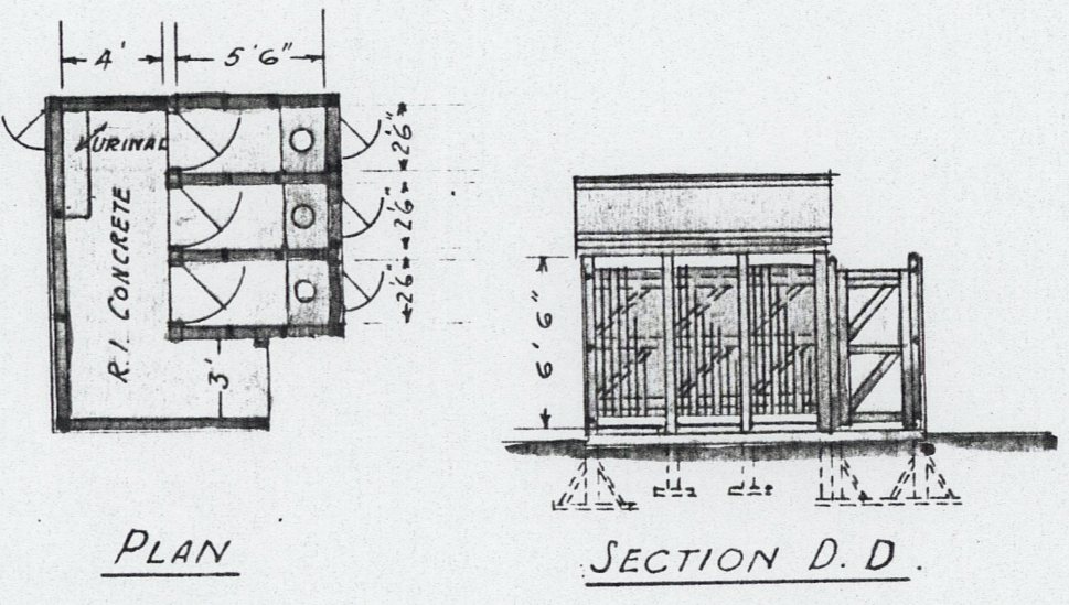
NEW LATRINES Scale 1/8"=1'0"
