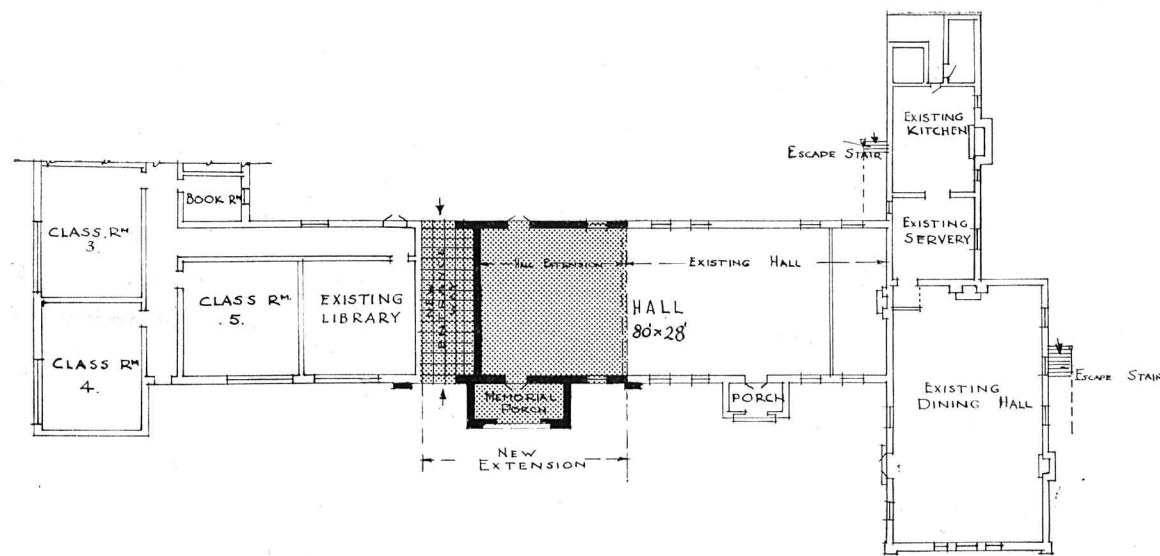
•GROUND FLOOR PLAN. SCALE - 1/16 TO 1'-0"
