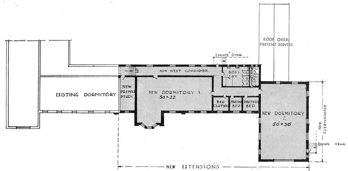
•FIRST FLOOR PLAN • SCALE - 1/16 TO 1'-0" •PROPOSED EXTENSIONS TO BALLARAT COLLEGE • H.LCOBURN, F.R.A.I.A - ARCHITECT 313, STURT ST - BALLARAT
