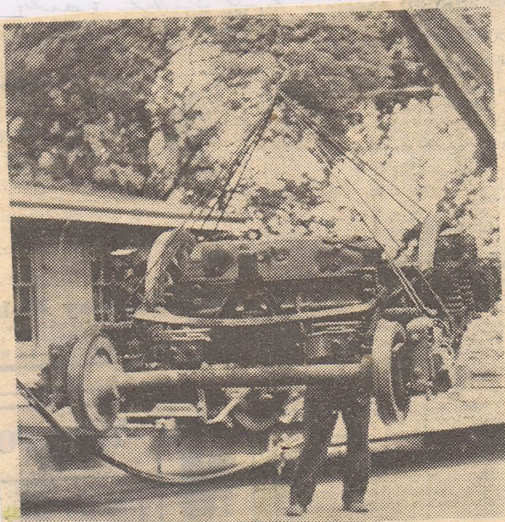
This new double bogie tram from Melbourne arrived in Ballarat yesterday for service in the city. It has a length of 45 feet, has a capacity for 44 and will give better service through quicker entry and exit. Bottom: Unloading one of the two bogies, the weight being approximately four tons.
