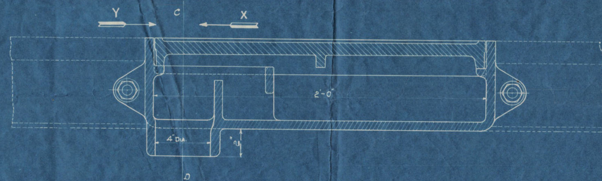
SECTIONAL ELEVATION ON AB
