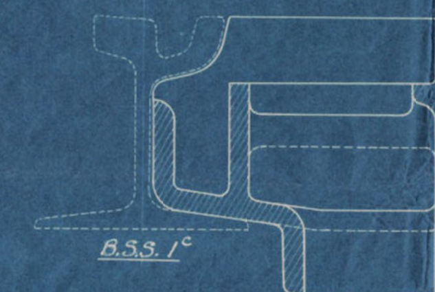
SECTION ON CD LOOKING IN DIRECTION OF Y (LID REMOVED)
