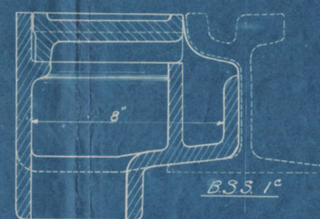
SECTION ON CD LOOKING IN DIRECTION OF X.
