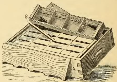
FIG. 57.—Super with sections and section holders in place: A, super; D, separator; F, sections; F, follower; G, wedge. (From Gleanings.)
