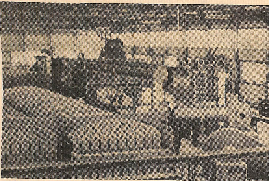
After being partially dried in small chambers, bricks are then manually stacked prior to being fired. At right of picture, conveyor-belt system is shown.
