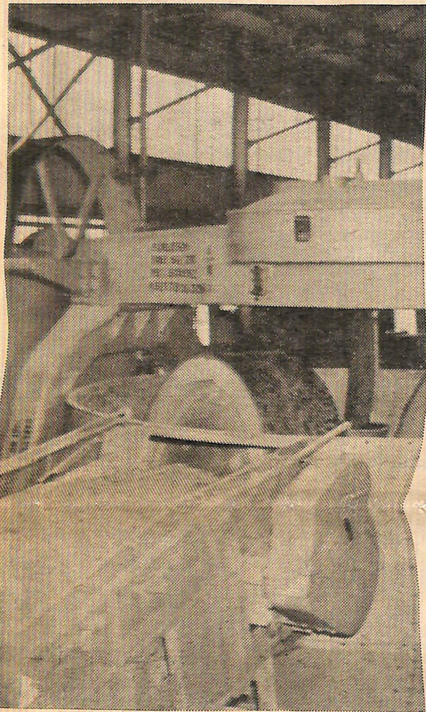
Other belts then move clay dust on towards the extruder, being gradually moistened as it moves along.
