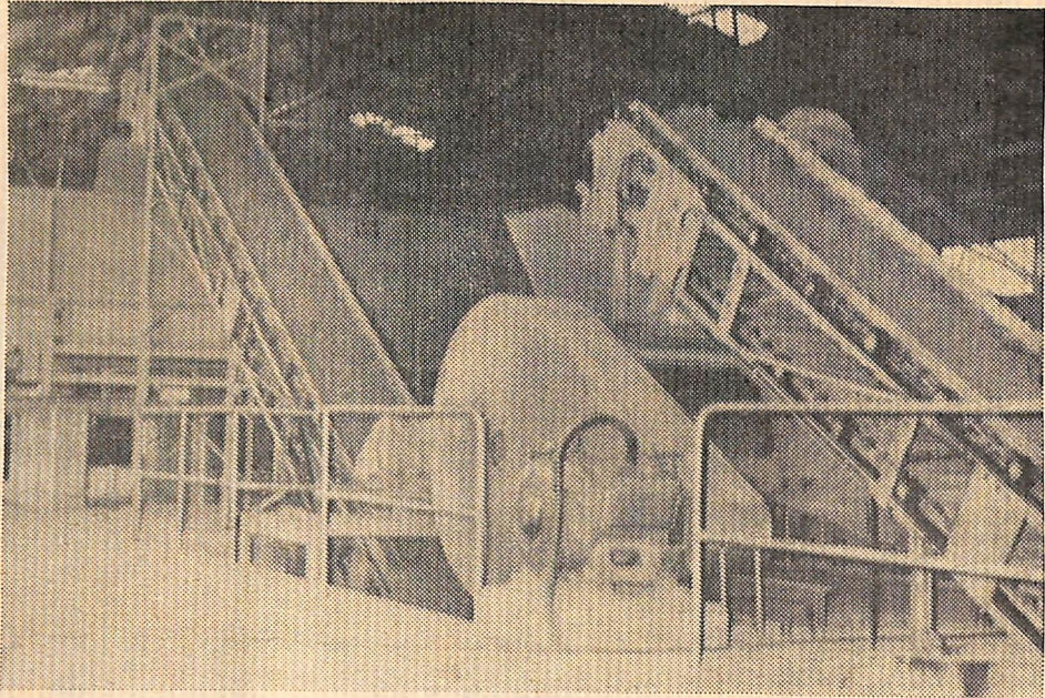
Top left: Truckloads of clay arrive from the pit and are dumped into a hopper.
