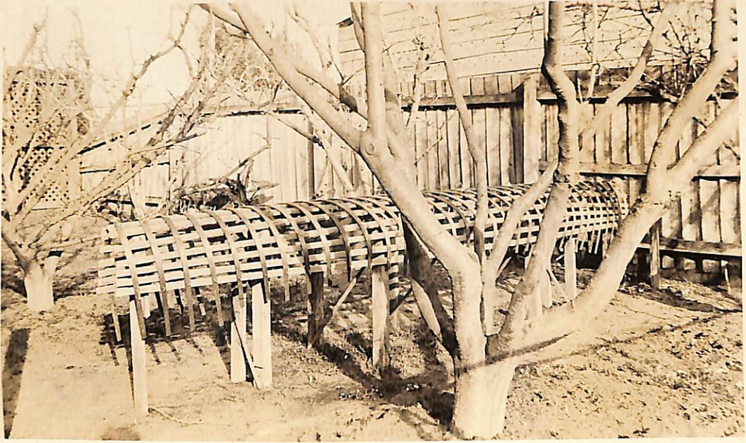
Ribs bent on mould.
