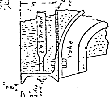
DETAIL AT YOKE. A. Scale: 1/2 inch to 1 ft.
