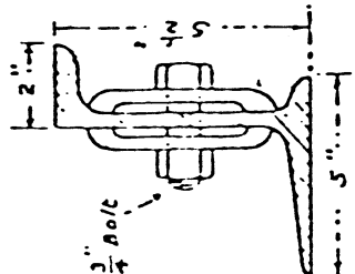
52 LB. SLOT BEAM Scale: 3 inches to 1 ft.
