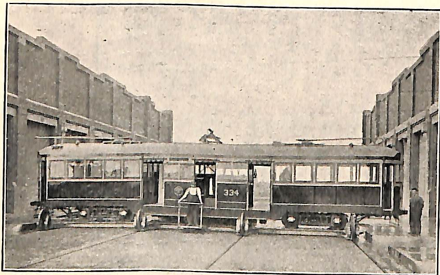
Fig. 2. Class W. Bogie Car on Traverser
