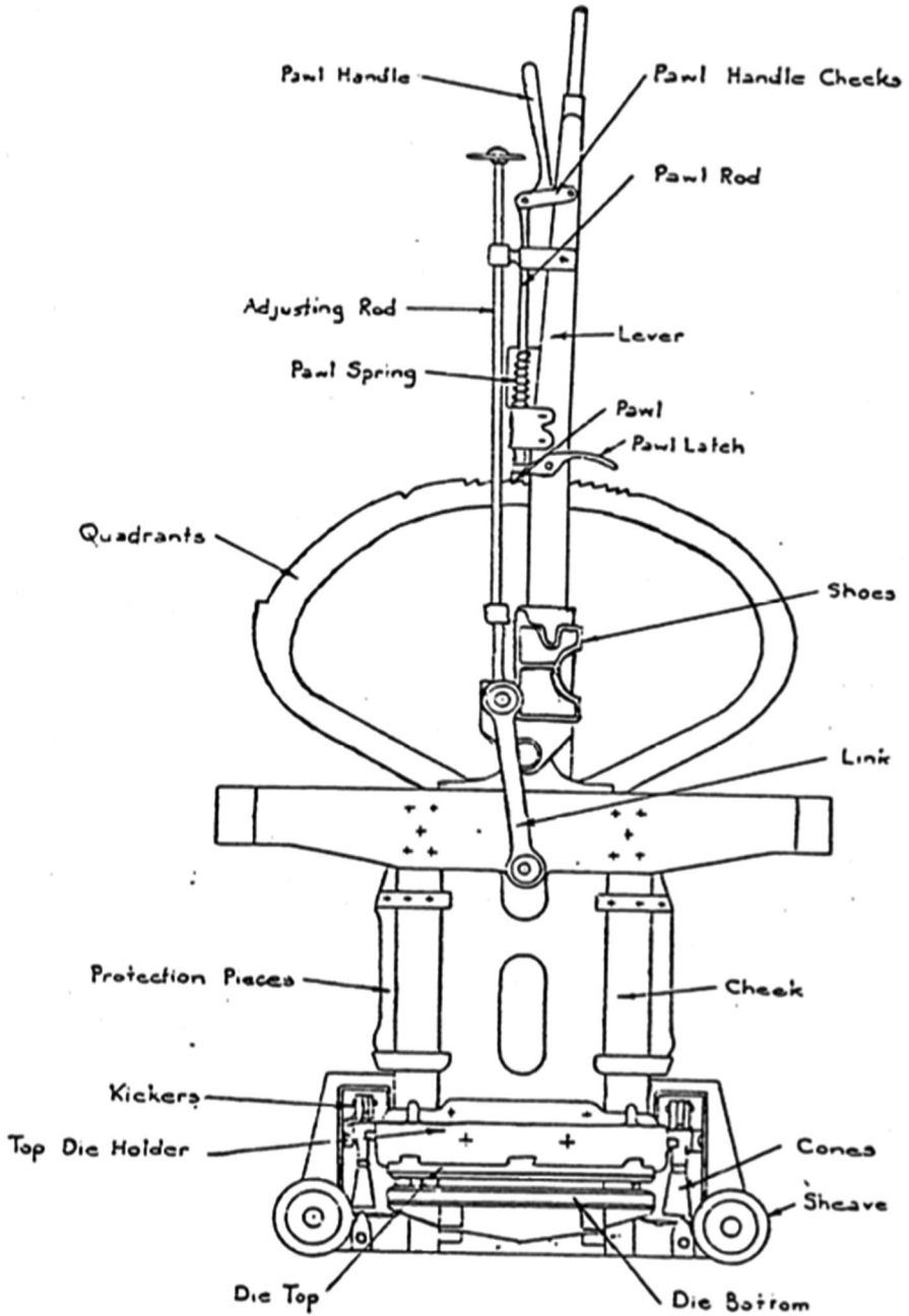
FIGURE 8 Diagram of grip. Grip jaws (dies) at bottom.
