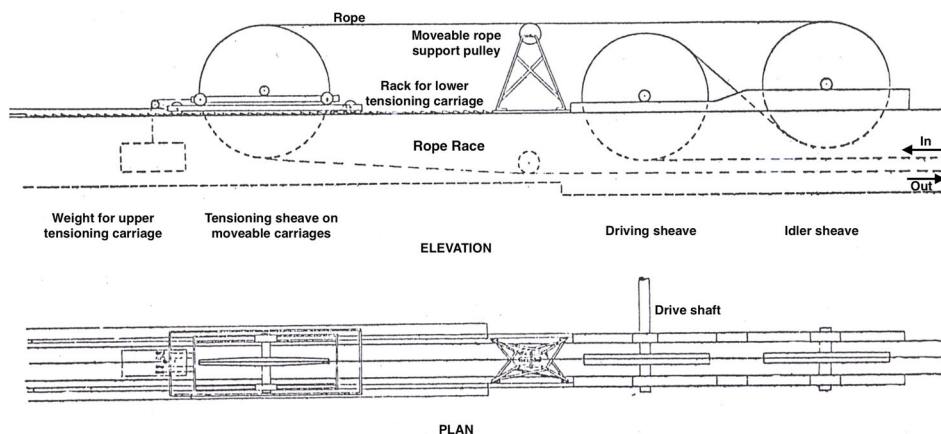
FIGURE 7 Diagram illustrating rope drive and tensioning with single drive sheave and idler sheave. From Pollock, c1950.
