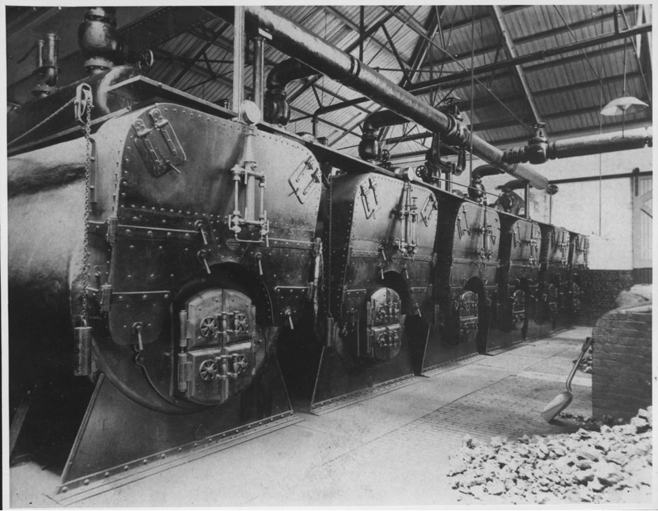
FIGURE 6 Interior of boiler room at Toorak engine house 1916. Photo SLV H36280/3.
