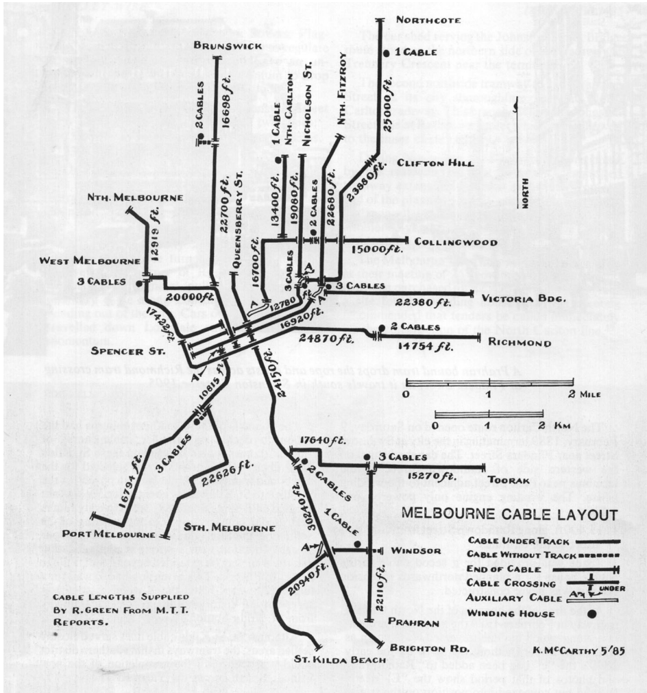
FIGURE 4 Schematic route diagram showing cable sections [Reproduced with permission from Australian Tramway Museum's Trolley Wire, No 221, Dec 1985].
