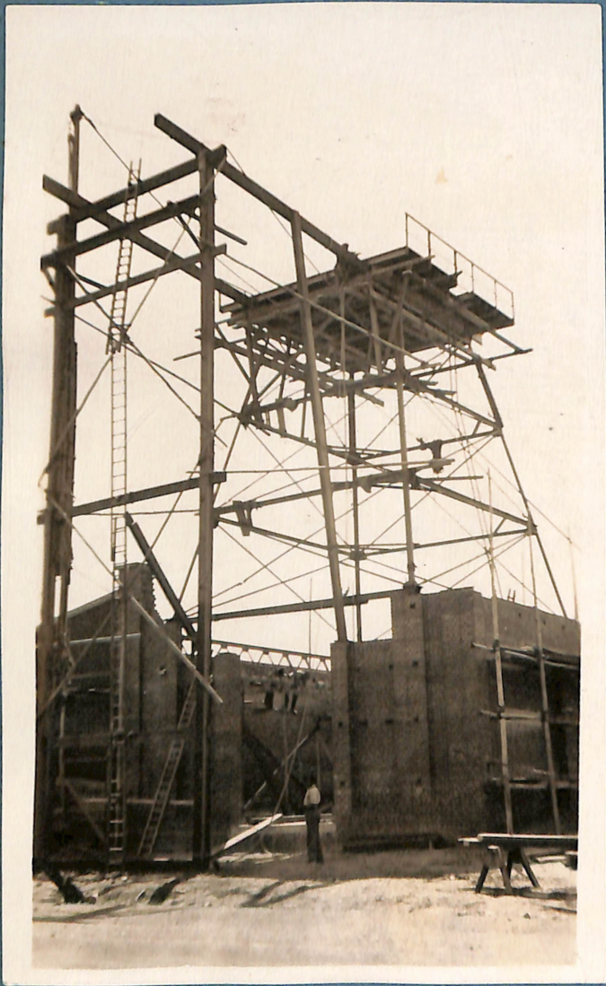
Elevated Tank South Melb. Depot.
