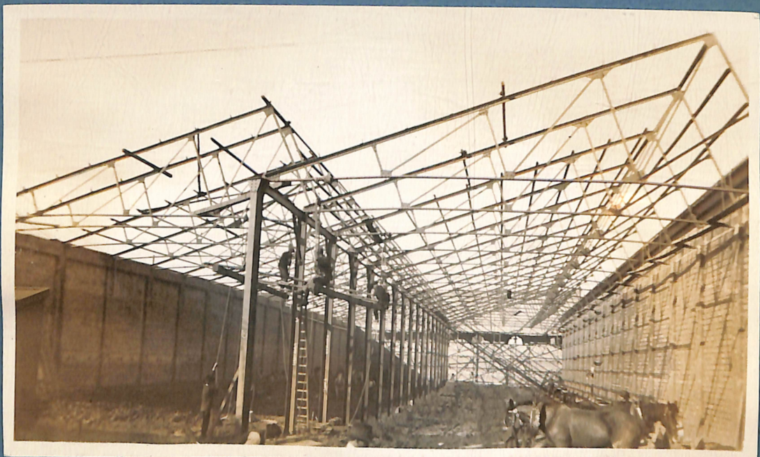
Extensions to Kew Car Depot
