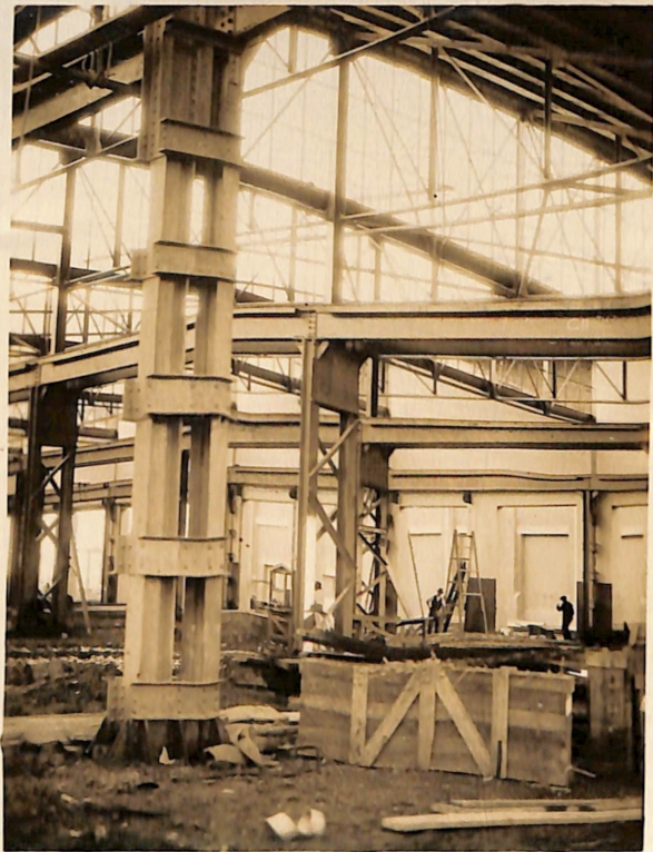
Portion of Truck Shop showing 3 Crane Bays
