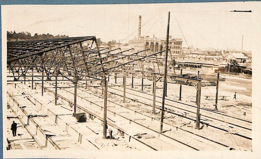
View of Reinforced Concrete Track Pits
