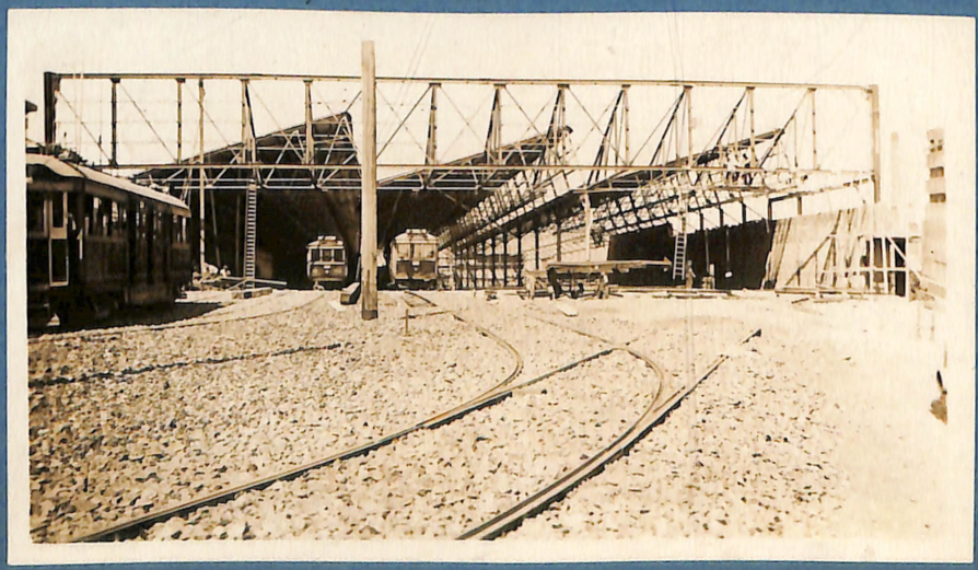
Views of 132' span Trussed Girder
