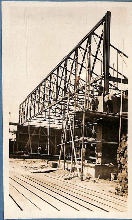
Views of 132' span Trussed Girder
